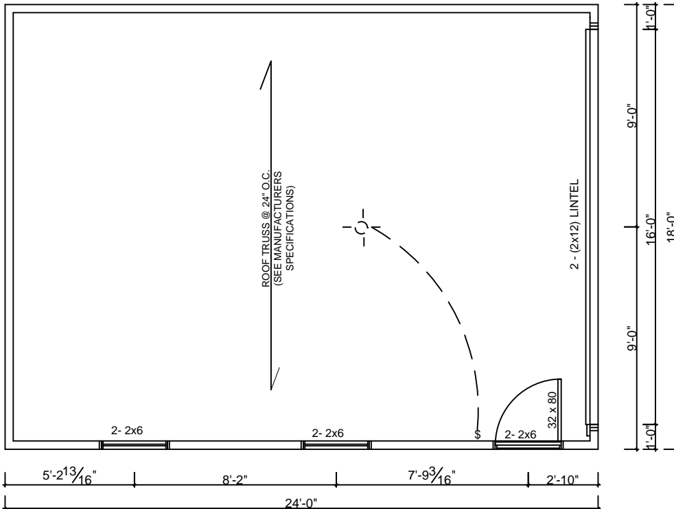
GARAGE PLAN
