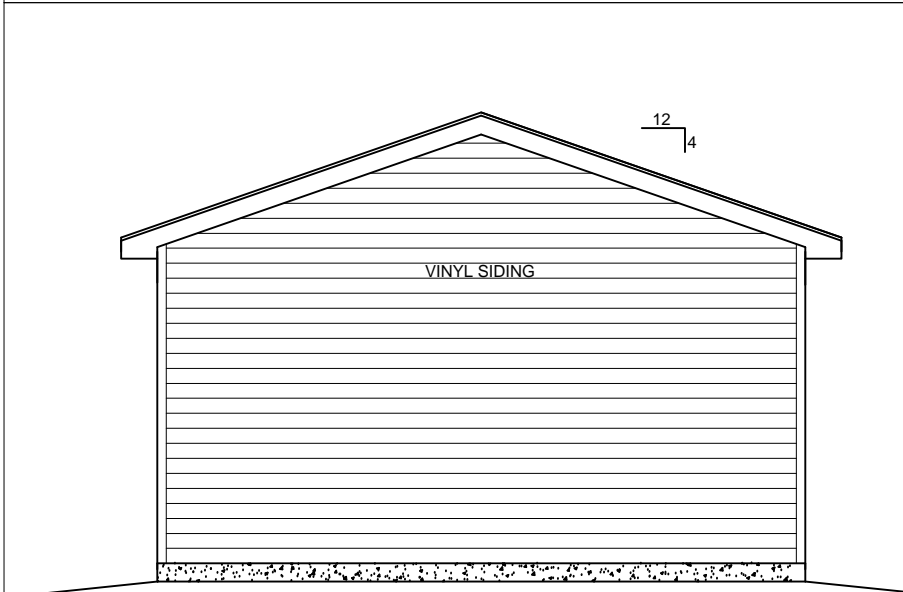
REAR ELEVATION
