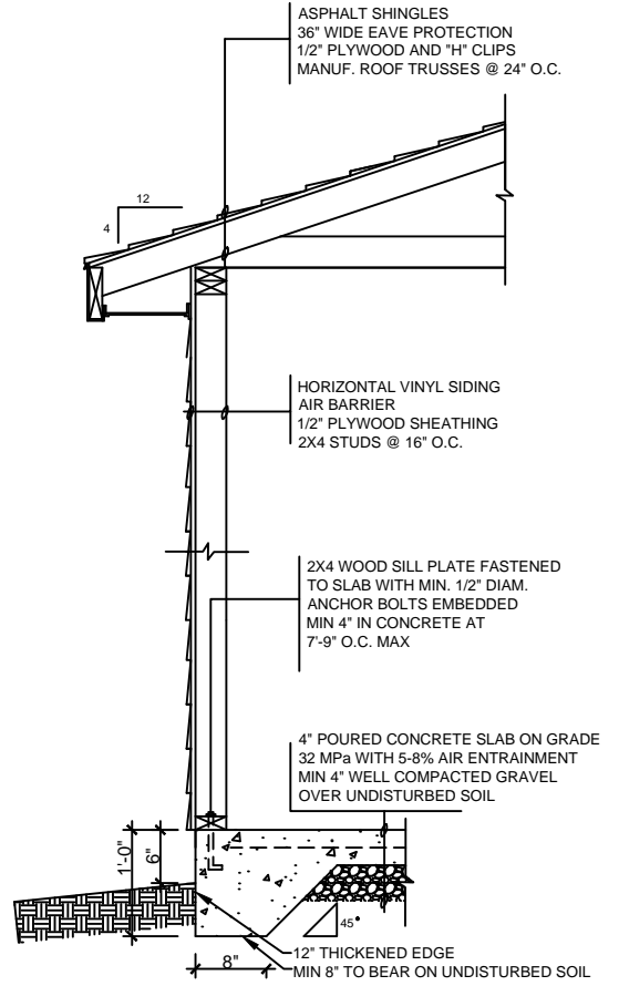
WALL SECTION
