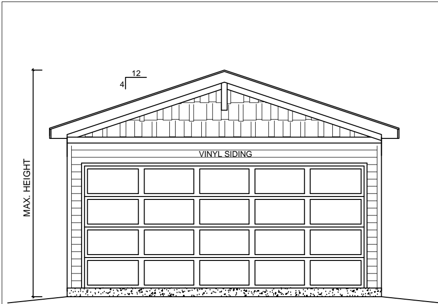
FRONT ELEVATION
