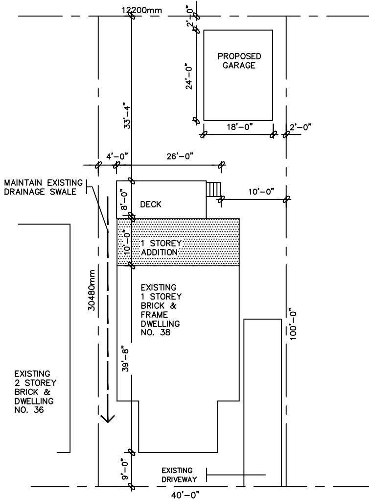
STREET NAME SITE PLAN
