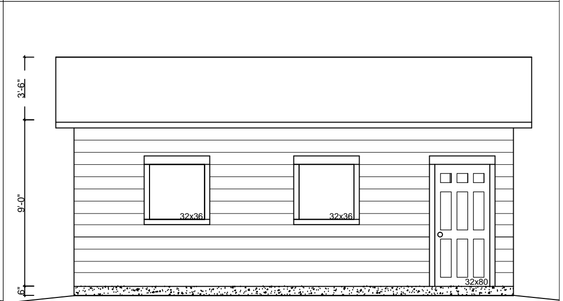
LEFT ELEVATION
