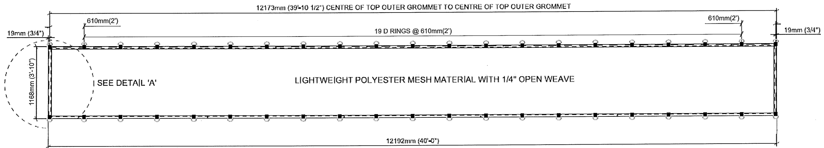
PLAN SCALE 1:40
