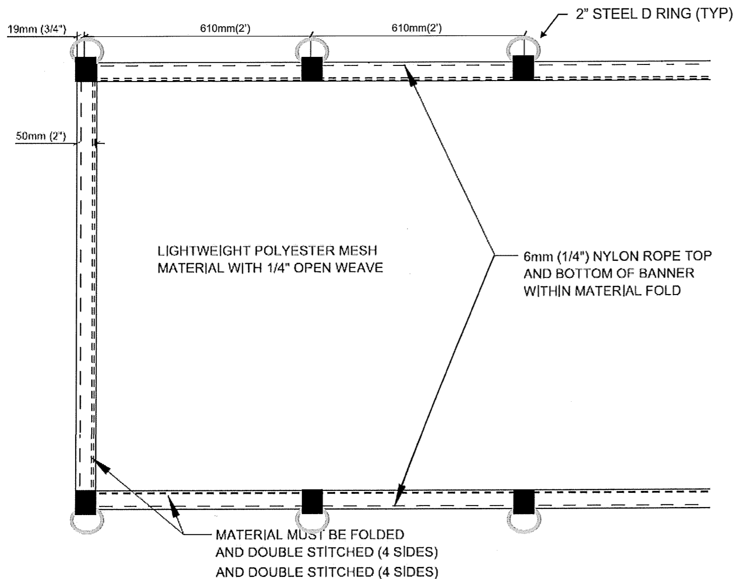
DETAIL-'A' SCALE 1:10
